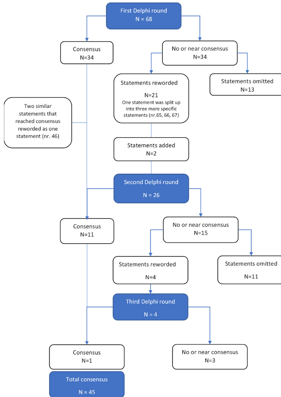
Fig. 3. Delphi process.
